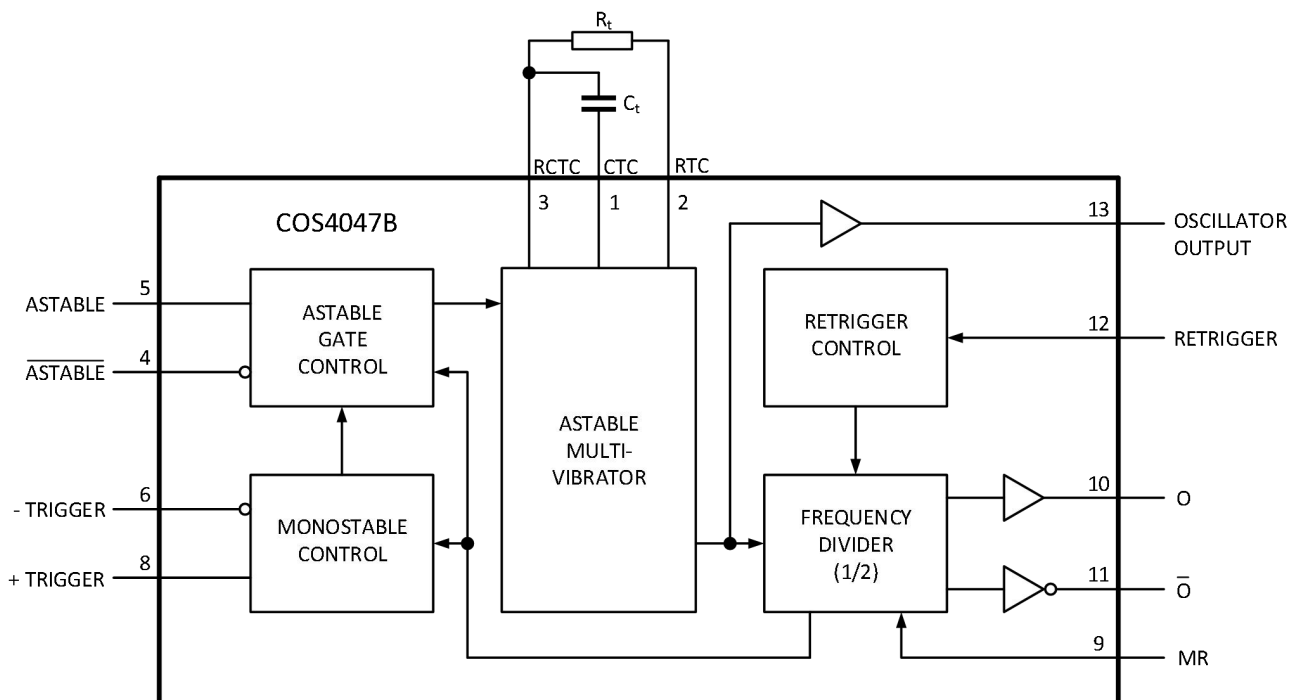
Figure 2. COS4047B Logic Block Diagram
