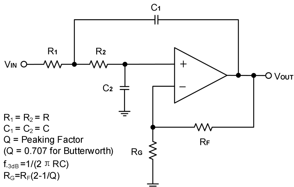
Figure 5. Two-Pole Low-Pass Sallen-Key Active Filter
