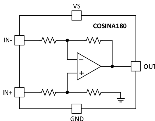
Simplified Schematic
